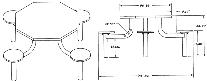
ISDT-4040-SS-XX
