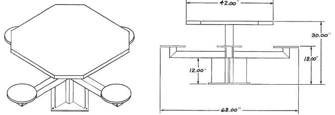
IPDT-4242-SS-XX
